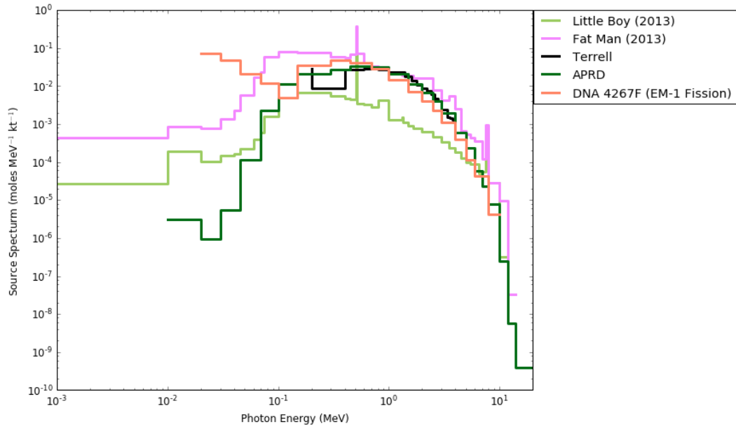
Figure 5. Photon spectra from fission sources
